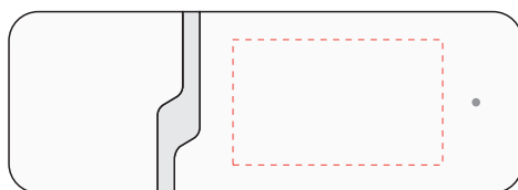
Front (Operation LED) Print size : 25mm x 15mm Pad Print
